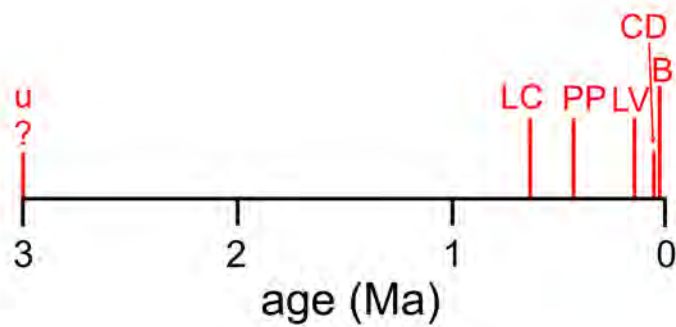
Figure 4. Known lakes in the GSL-BB larger than modern GSL during the past 3 Ma. Chronologic data are from the Burmester core for the Bonneville, Little Valley, Pokes Point, Lava Creek, and unnamed lake cycles (Oviatt and others, 1999; unpublished information); the age of the CD lake cycle is from Kaufman and others (2001). The X axis of the graph marks the approximate elevation of modern GSL (~1280 m), and the vertical scale, which represents the relative maximum elevations of lakes, is not shown on the figure because insufficient information is available for most lake cycles. Approximations of the upper elevation limits of the CD and LV lake cycles are based on outcrops of lacustrine sediment. The upper elevation limits of the PP and LC lake cycles are interpreted as being similar to that of the LV lake cycle. The elevation of the unnamed lake cycle at about 3 Ma is unknown, but based on the ostracode fauna in sediments of that age from the Burmester core, the lake probably did not rise higher than the CD lake cycle. B = Bonneville, CD = Cutler Dam, PP = Pokes Point, LC = Lava Creek, u = unnamed lake cycle.
